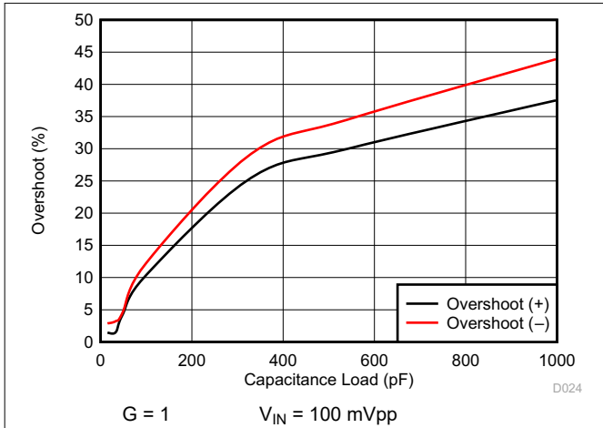
Figure 6-18. Small Signal Overshoot vs Capacitive Load
