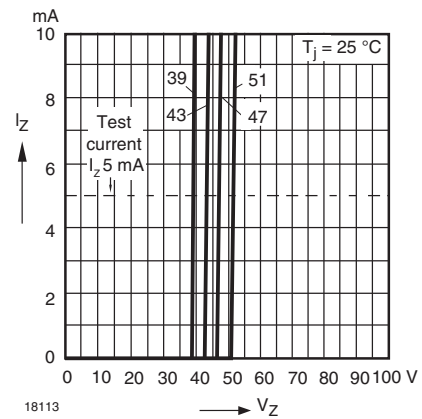
Fig. 16 - Breakdown Characteristics
