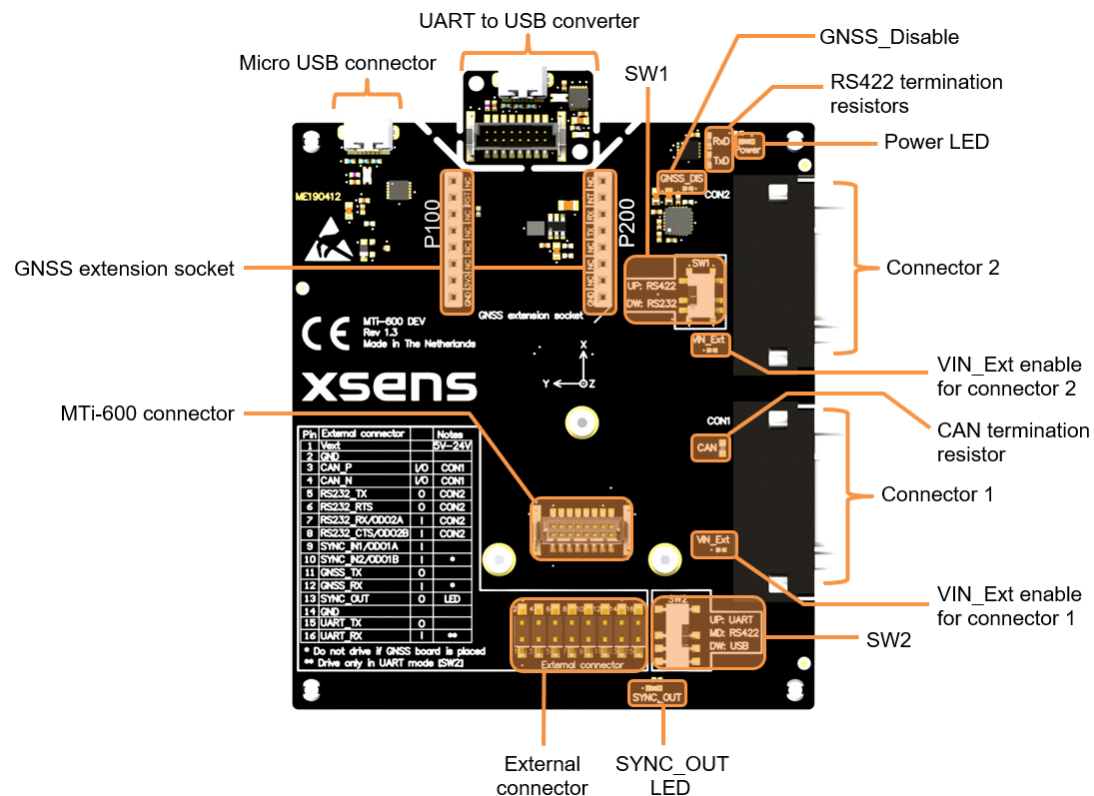
Figure 7: MTi 600-series Development Board overview with connector designators
