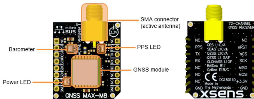
Figure 10: Top view (left) and the bottom view (right) of the GNSS daughter card
