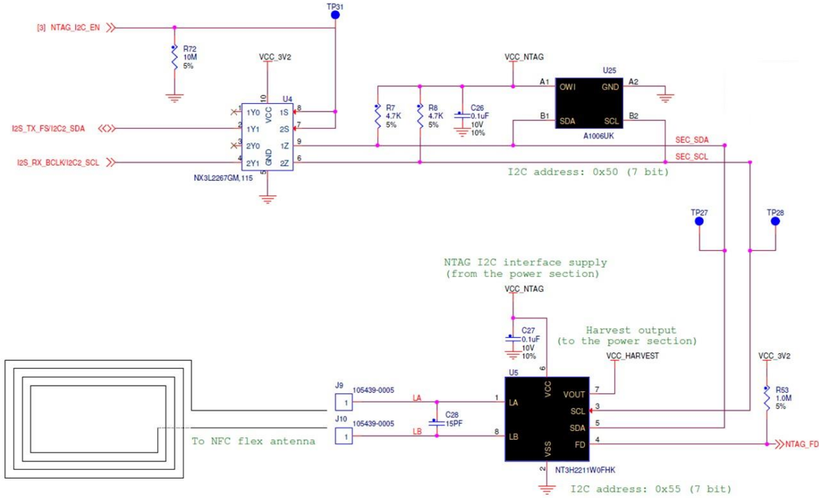
Figure 92. NT3H2211 NFC Tag
