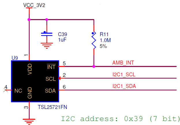
Figure 88. TSL25721FN Ambient Light Sensor
