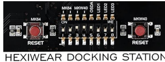
Figure 185. Docking Station Jumper Switch configuration to debug KW41Z
