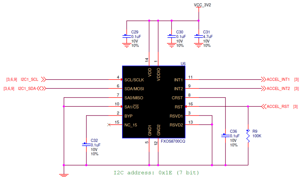
Figure 83. FXOS8700CQ Accelerometer and Magnetometer
