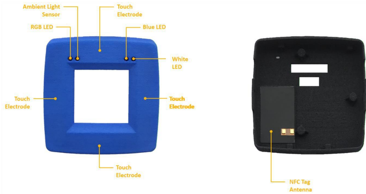
Figure 74. Rapid IoT touch-board and casing callout
