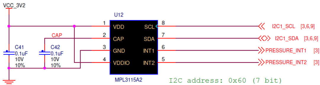
Figure 85. MPL3115A2 Barometric Pressure and Temperature Sensor
