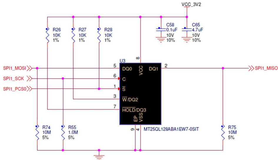
Figure 94. MT25QL128ABA1EW7 Serial NOR Flash
