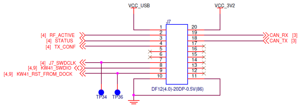
Figure 103. 20-pins extension connector
