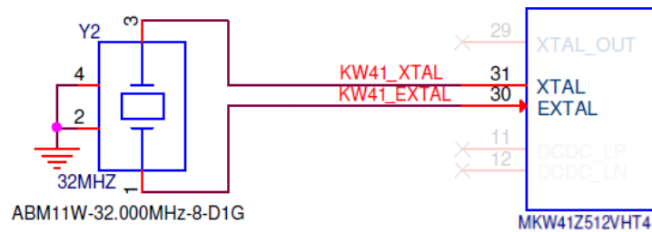
Figure 81. KW41Z Clock source
