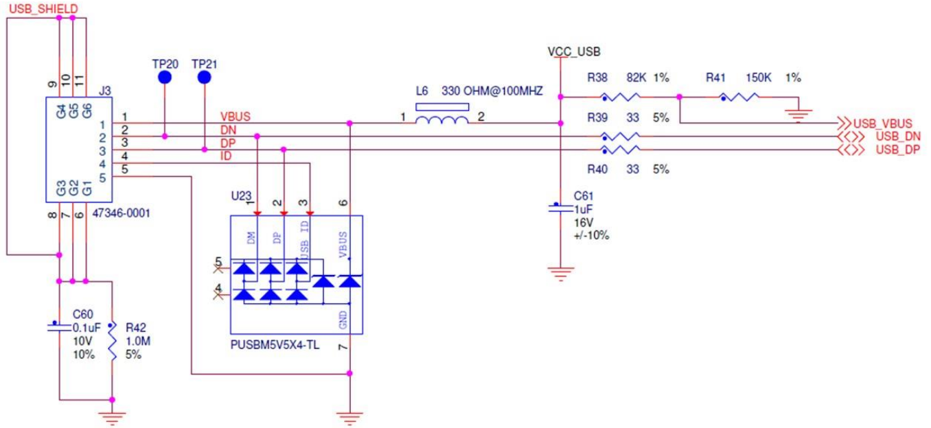
Figure 101. K64F USB interface
