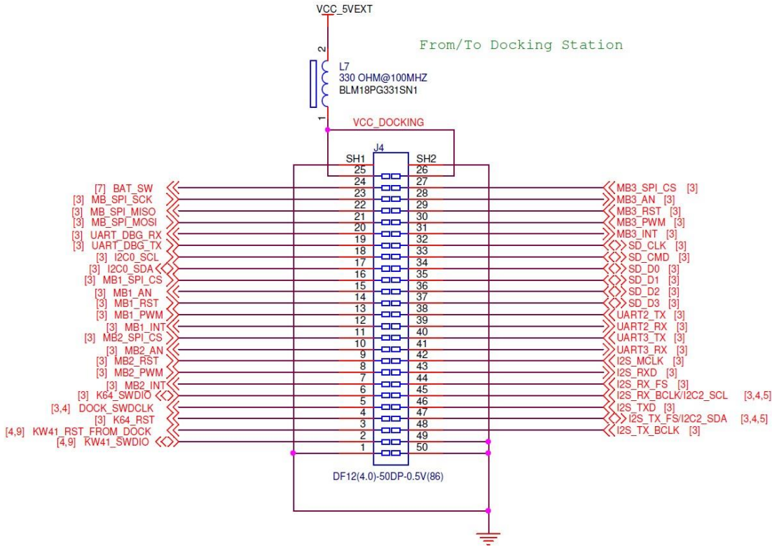
Figure 102. 50-pins extension connector
