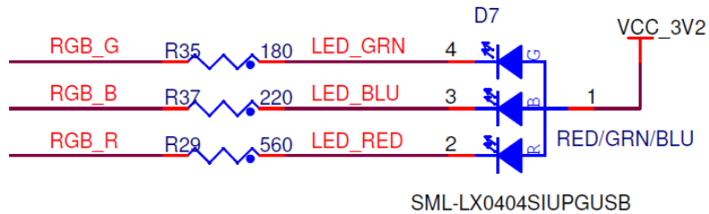
Figure 95. SML-LX0404SIUPGUSB RGB LED
