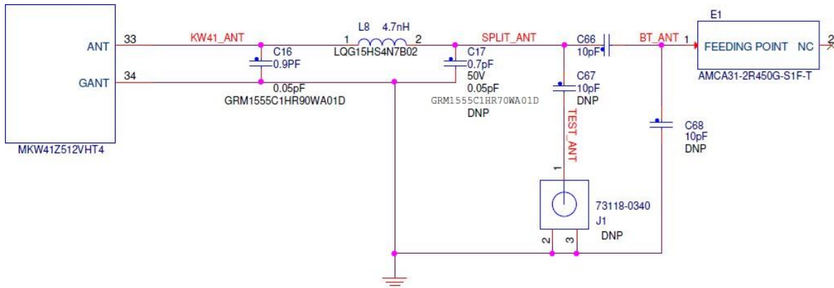
Figure 75. KW41Z RF circuit
