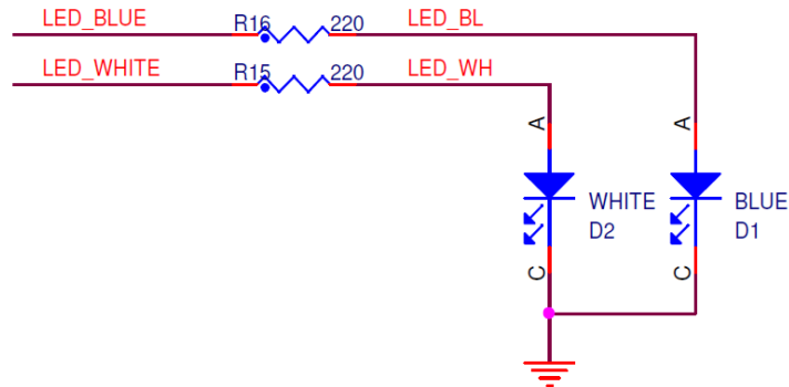
Figure 96. Connectivity Status LEDs
