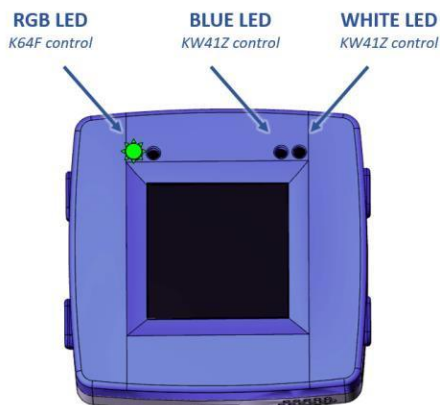
Figure 162. K64F Recovery LED
