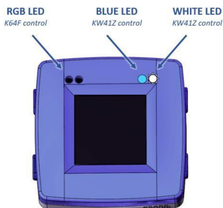
Figure 164. KW41Z Recovery LED
