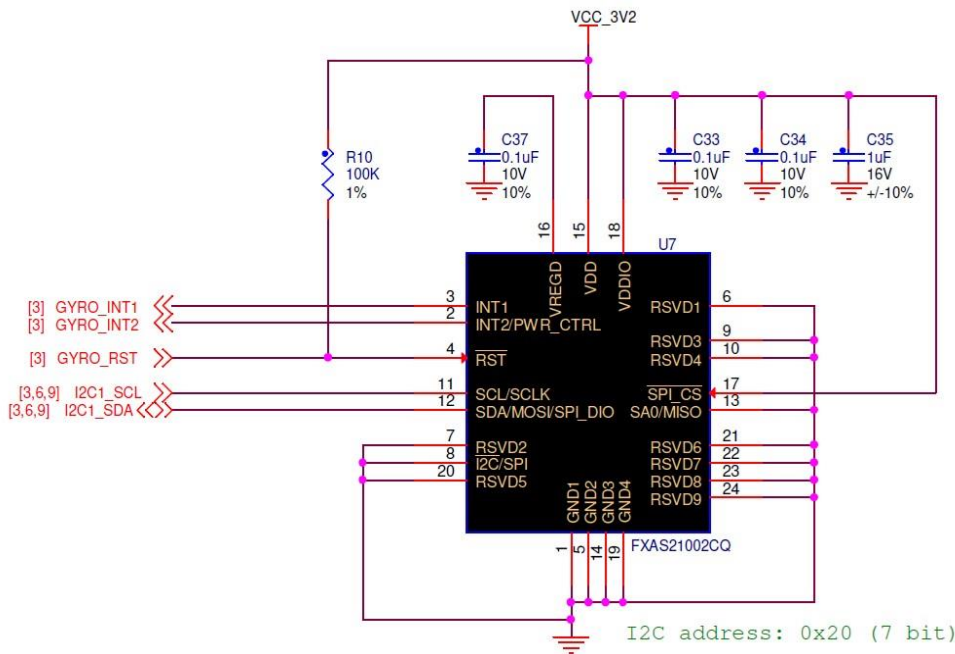
Figure 84. FXAS21002CQ Gyroscope
