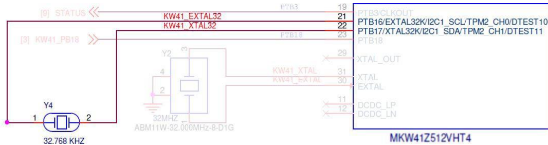
Figure 82. KW41Z Clock source
