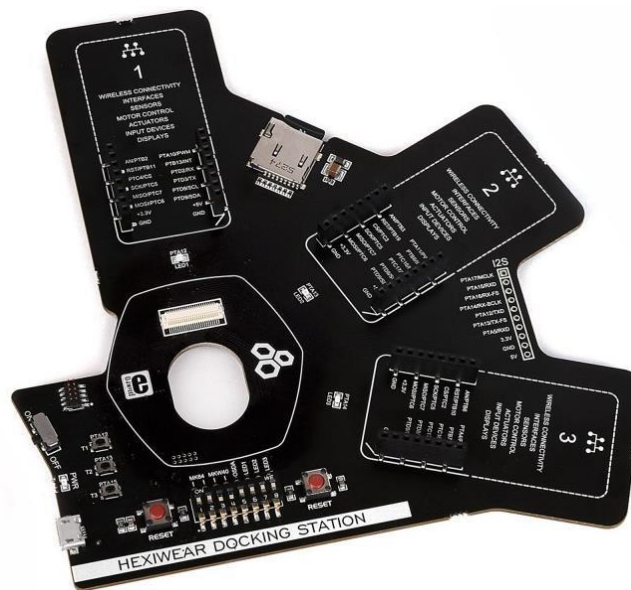
Figure 105. MikroElektronika Docking-station
