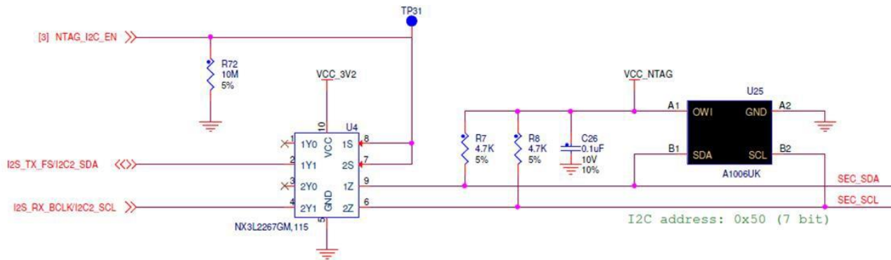
Figure 90. A1006 Security Chip
