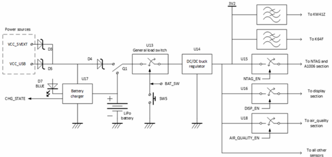
Figure 78. Power supply overview
