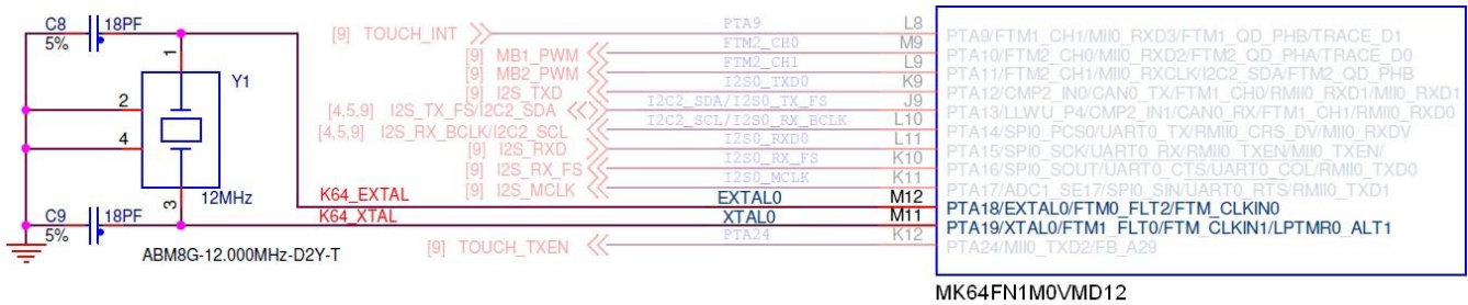
Figure 80. K64F Clock source
