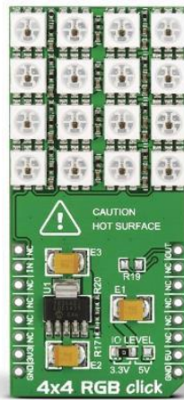
Figure 111. 4X4 RGB Click™
