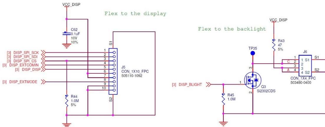
Figure 89. Connectors to the LCD display
