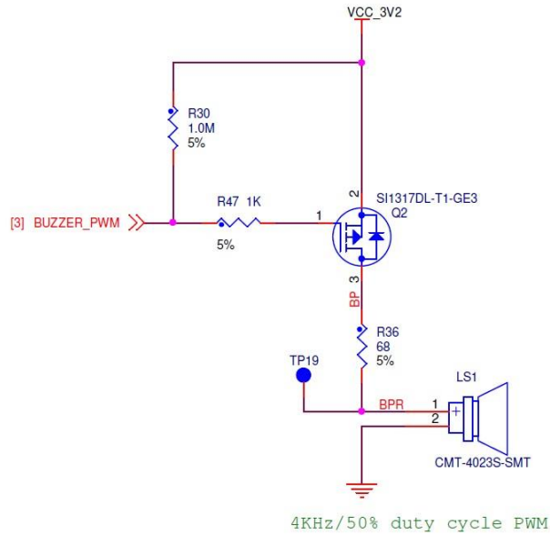
Figure 97. CMT-4023S-SMT Buzzer
