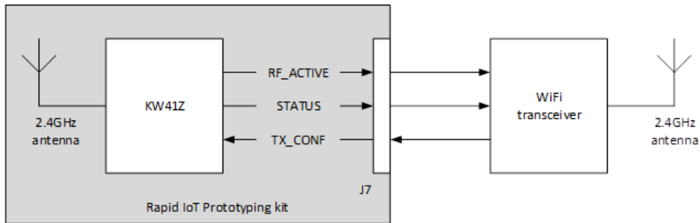
Figure 76. KW41Z CoExistence interface
