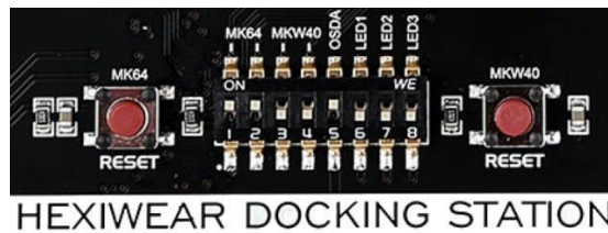
Figure 183. Docking Station Jumper Switch configuration to debug K64F
