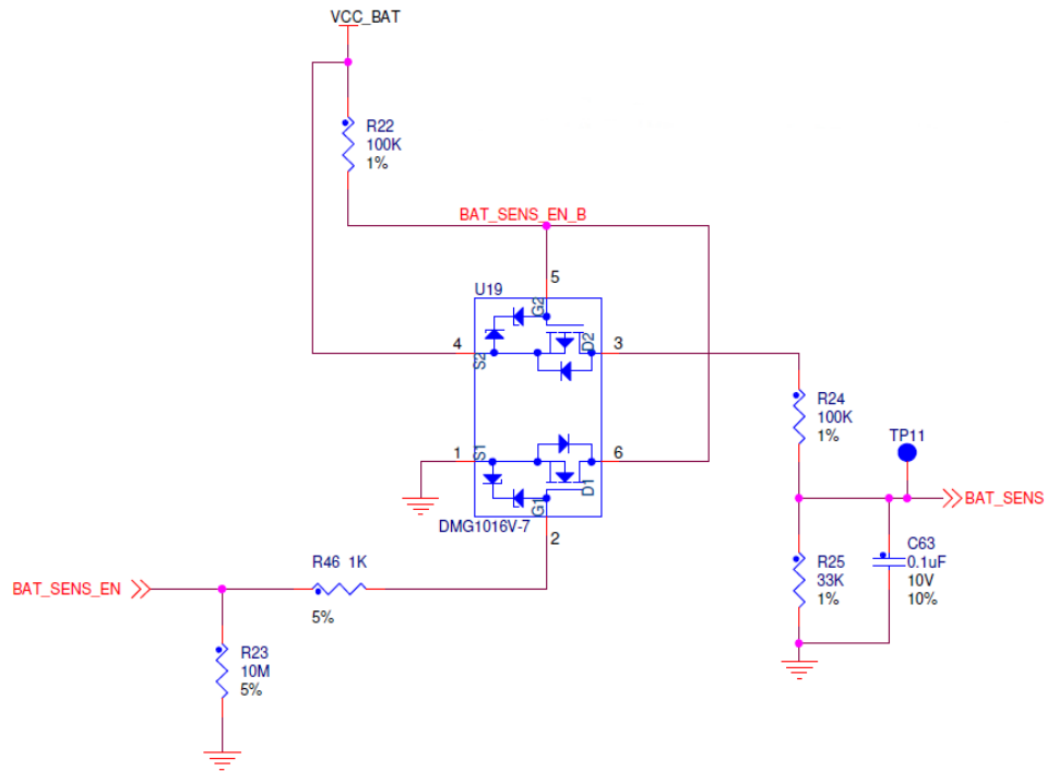
Figure 79. Battery sensing implementation
