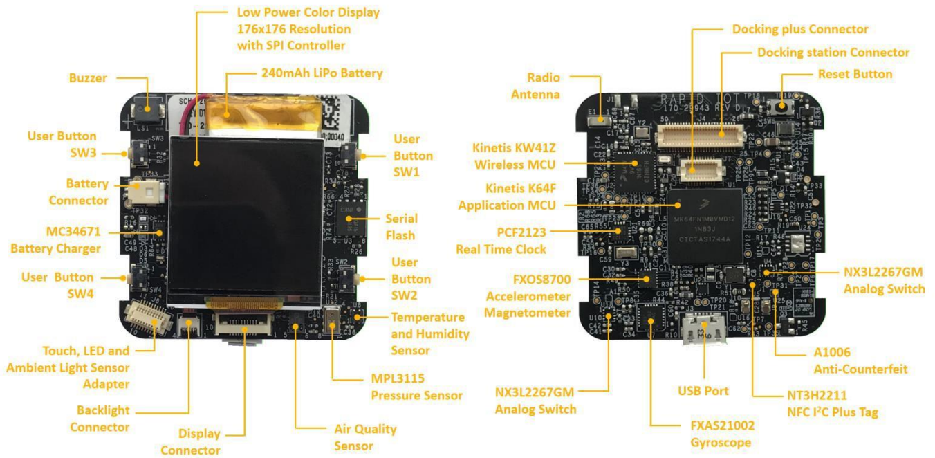
Figure 73. Rapid IoT main-board callout
