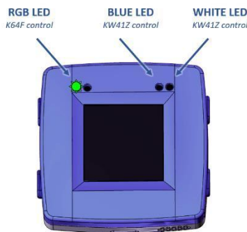
Figure 48. USB Programming LED
