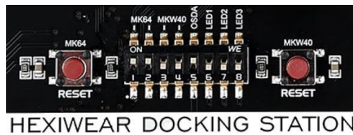
Figure 109. Docking Station Jumper Switch configuration to debug K64F
