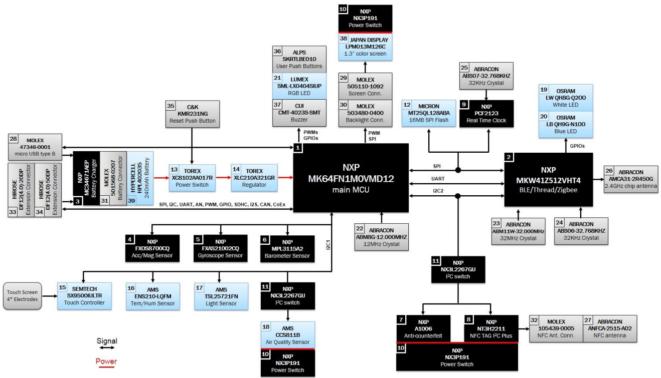
Figure 72. SLN-IOT-NODE block diagram
