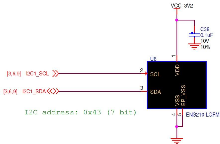
Figure 86. ENS210 Humidity and Temperature Sensor
