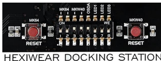
Figure 173. Docking Station Jumper Switch configuration to debug KW41Z
