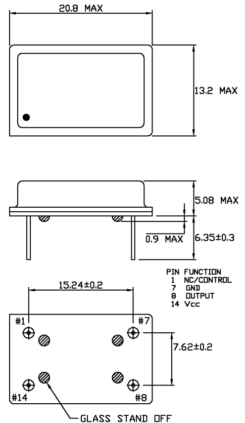
STYLE 1 FULL SIZE 14 PIN DIP
