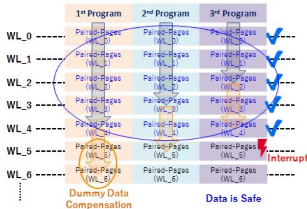
Figure 3-14: Dummy Data Compensation
