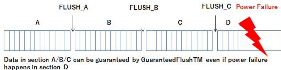
Figure 3-13: Timing of Triggering GuaranteedFlush™
