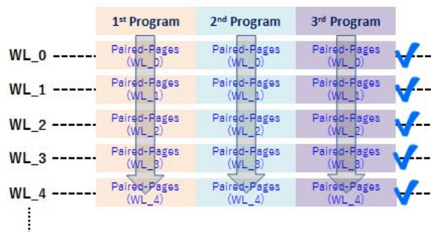
Figure 3-11: Programming Operation of TLC Flash
