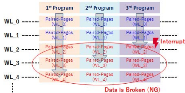
Figure 3-12: Power Loss during Data Programming
