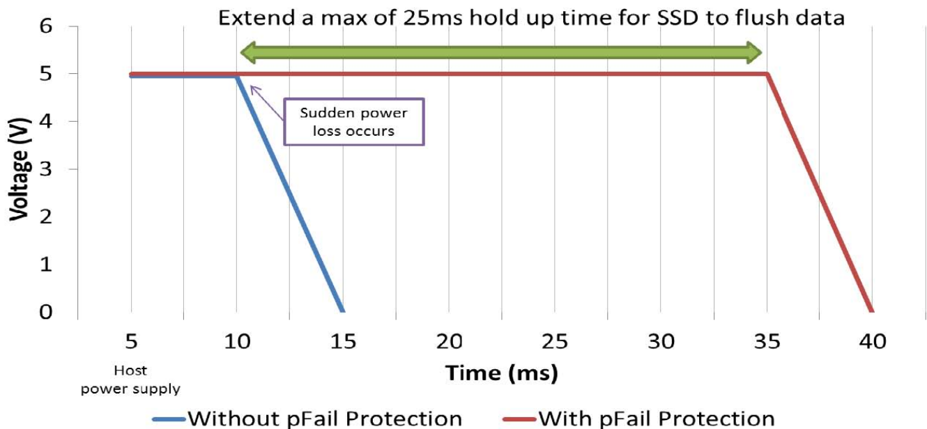
Figure 2-1: 512GB example of Controller/DRAM Capacitive hold-up time
