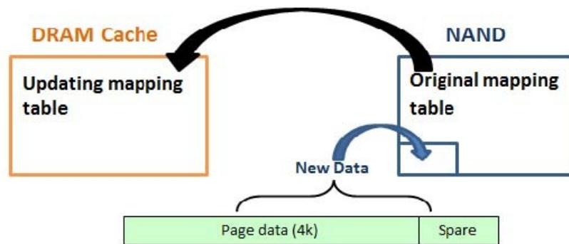
Figure 3-8: Rebuilding Metadata Mapping Table
