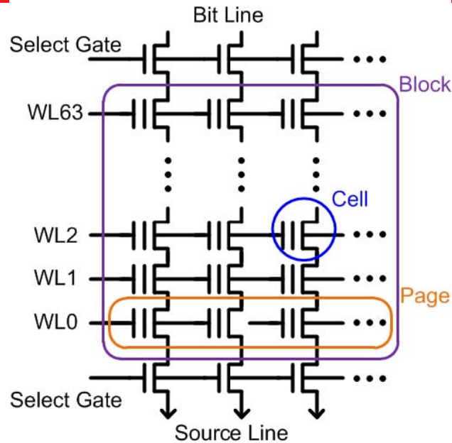
Figure 3-9: NAND Composition in Transistor Level
