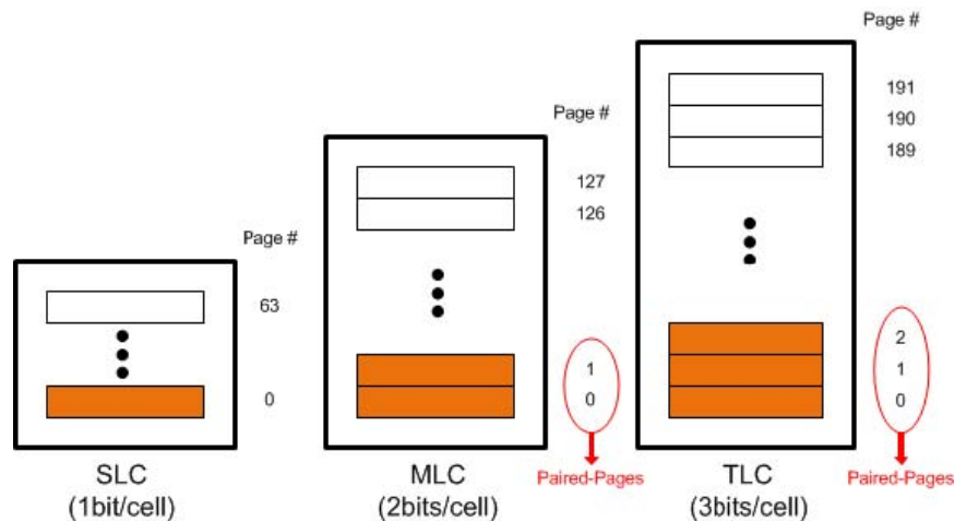
Figure 3-10: Paired-Pages
