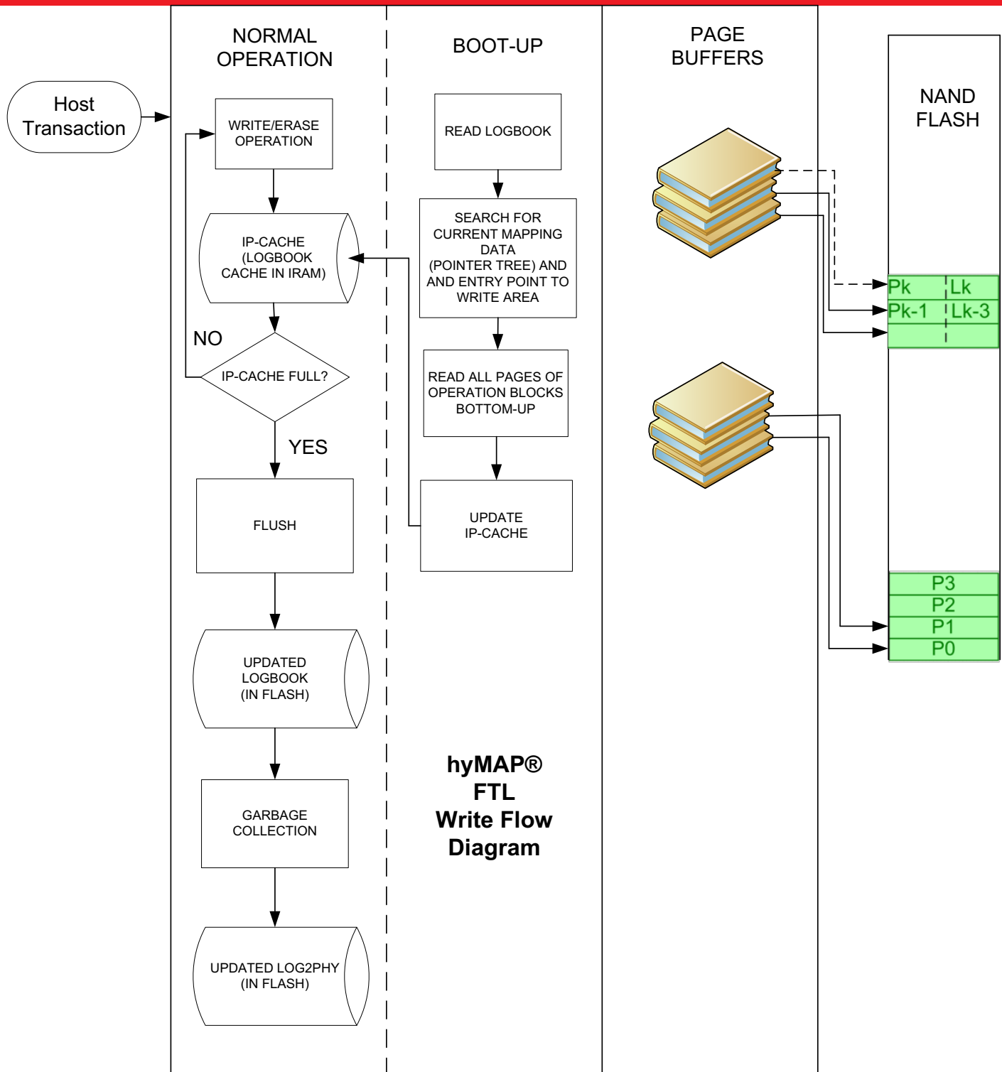
Figure 4-1: hyMAP® FTL Write Flow Diagram
