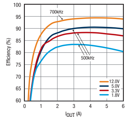
XR79206 Efficiency
