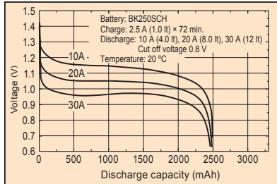
Discharge characteristics
