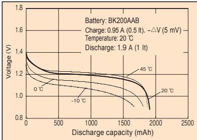
Discharge characteristics
