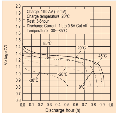
Discharge characteristics
