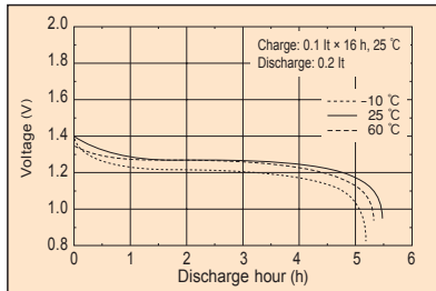
Discharge characteristics
