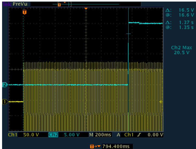
Figure 11: Turn on delay time measured waveform@90Vac/50Hz,full load
