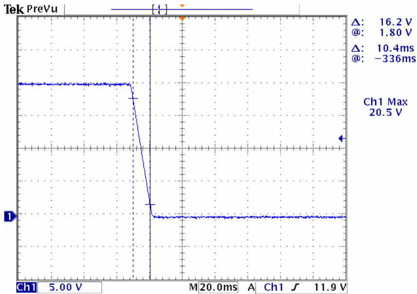
Figure 14: Fall time measured waveform@90Vac/50Hz,full load
