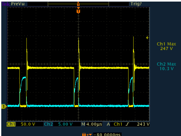
Startup with Output short, Vds wave form@90Vac/50Hz,
