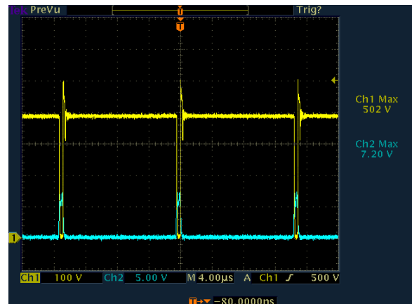
Output short, Vds wave form@264 Vac/50Hz,
