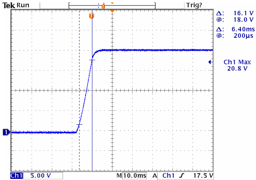
Figure 13: Rise time measured waveform@90Vac/50Hz,full load
