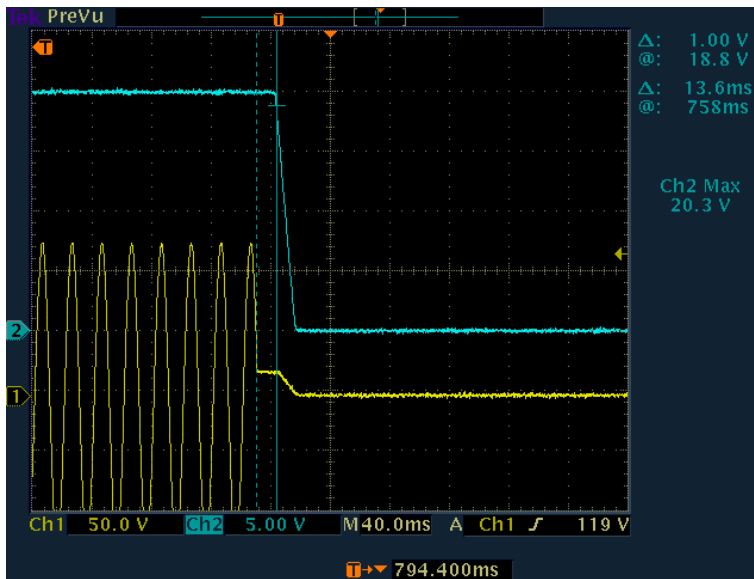
Figure 12: Hold on delay time measured waveform@90Vac/50Hz,full load
