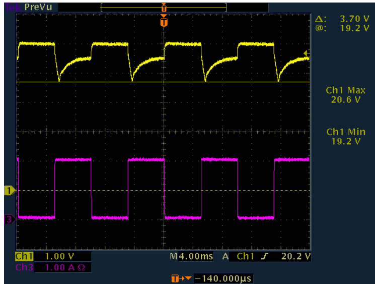
Figure 10: Output voltage waveform under Dynamic test@90Vac/50Hz,full load
