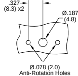
Mounting Hole Detail
