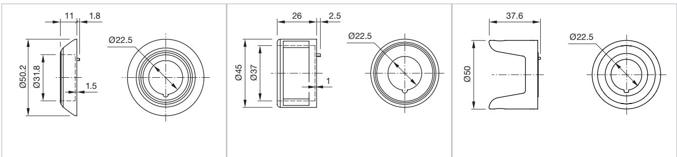
Dimensions [mm] for Part No. 84-902, 84-902A 84-902B, 84-902C
