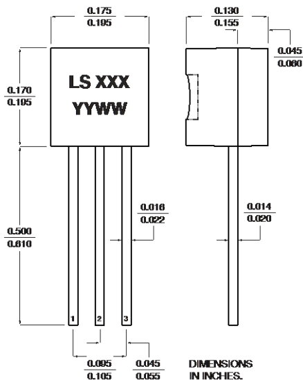
TO-92 3 Lead
