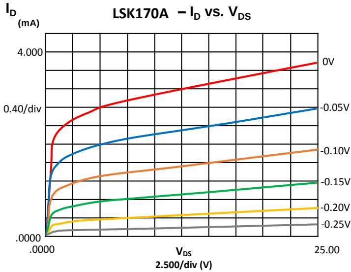
Output Characteristics
