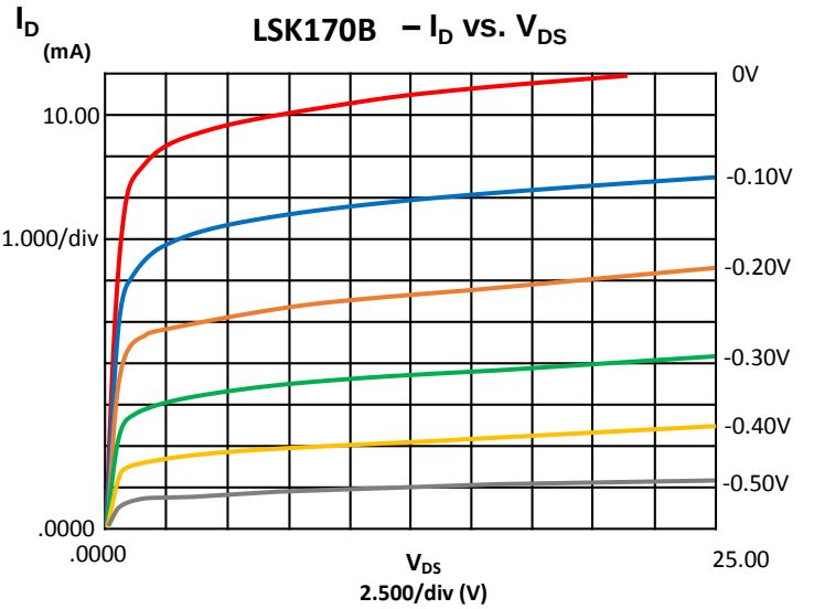
Output Characteristics
