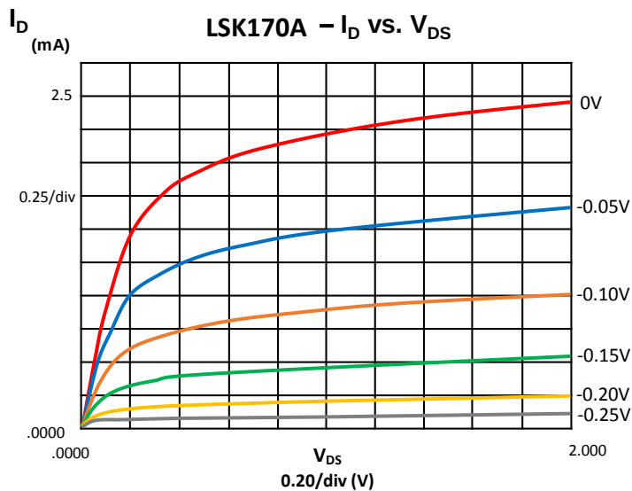
Operating Characteristics
