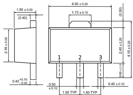
SOT-89 3 Lead
