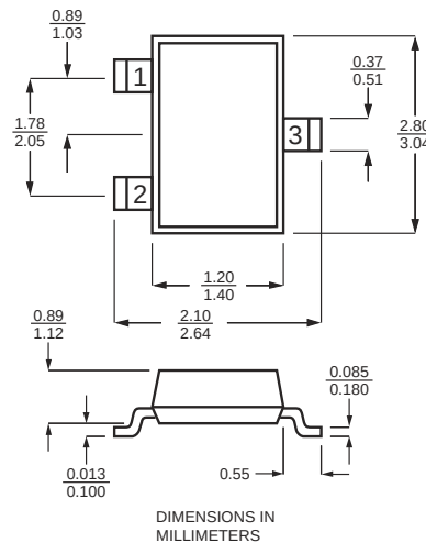
SOT-23 3 Lead
