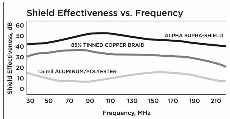
Figure 2. Foil-braid shielding yields the best shielding effectiveness
