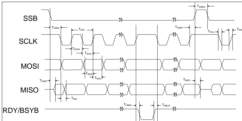
Figure 11-1 SPI Timing
