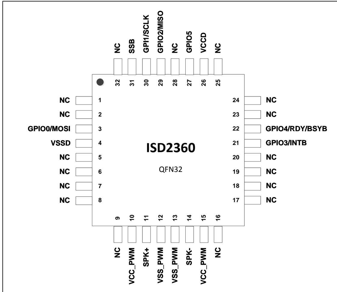
Figure 2-1 ISD2360 QFN 32-Lead Package
