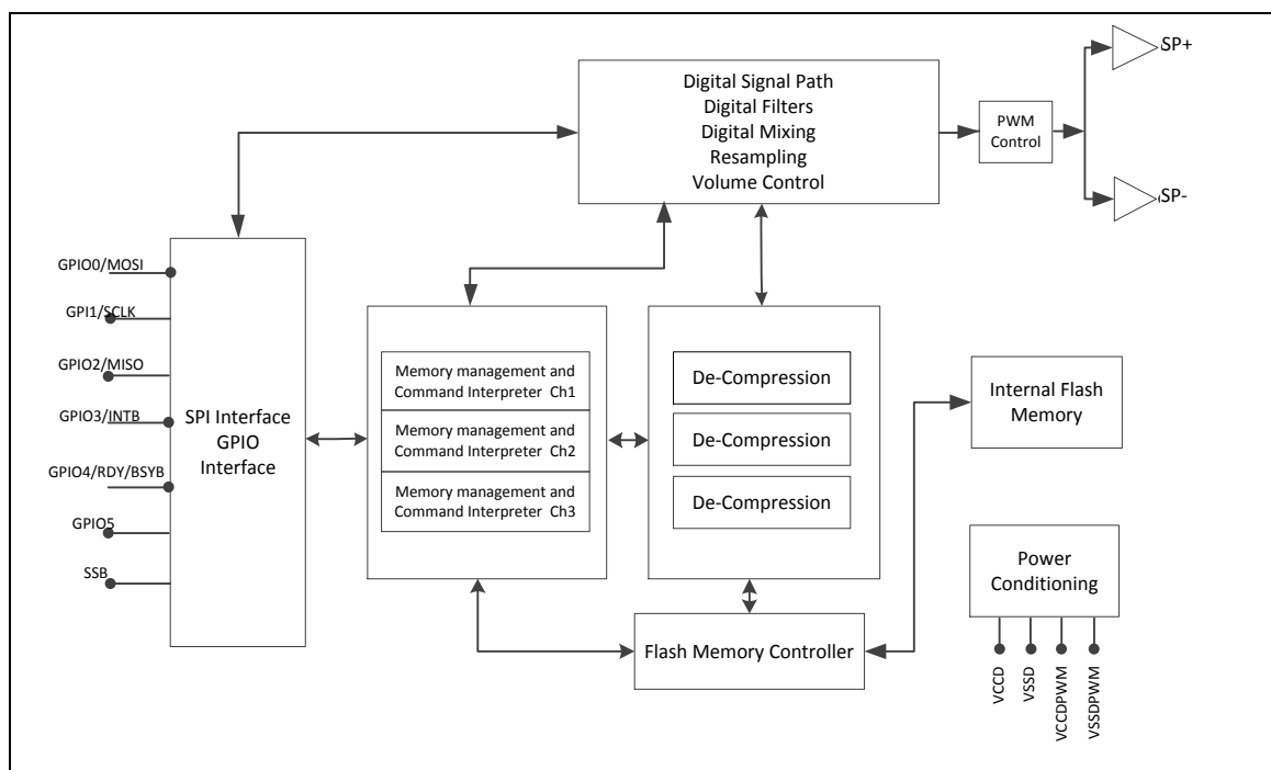
Figure 3-1 ISD2360 Block Diagram
