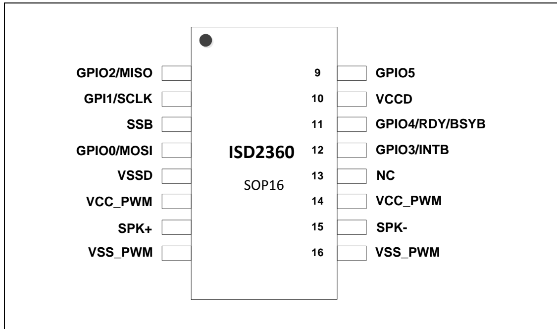
Figure 2-2 ISD2360 SOP 16-Lead 300 mil Package
