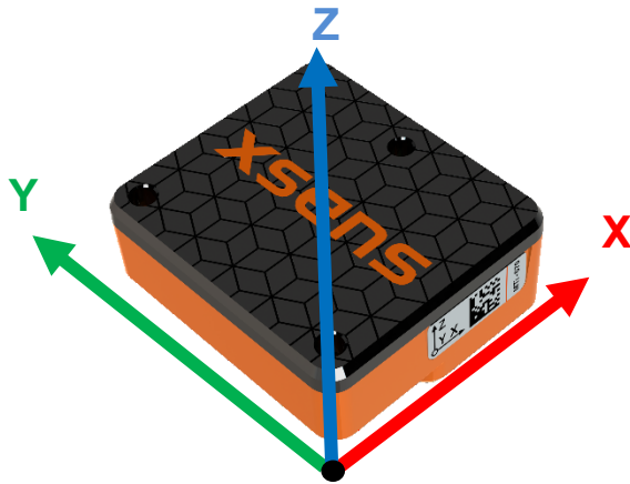
Figure 8: Default coordinate system of MTi 600-series
