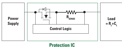
Protection IC Function Block Diagram
