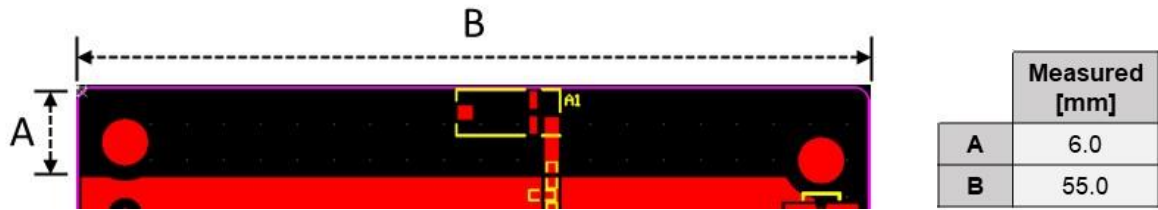
Figure 18 - Sanity check of the antenna clearance area
