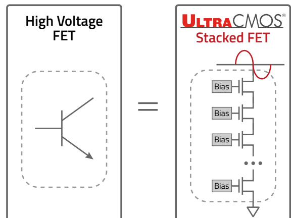
FET stacking is a very efficient way to handle power using low voltage devices
