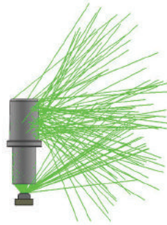
Optical simulation of VCC's custom designed light pipe design
