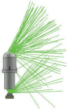
Optical simulation of customers current light pipe design
