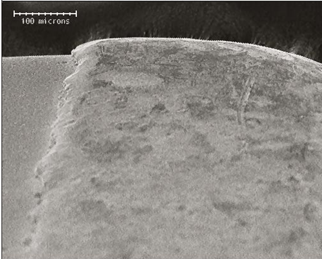
160S41W475KT4 #514-5389, 1000 cycles
