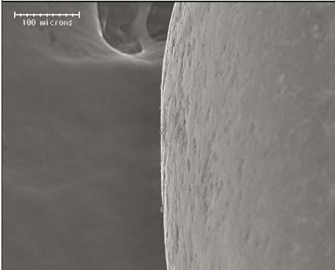
500R15W473KV4 #514-7276, 1000 cycles
