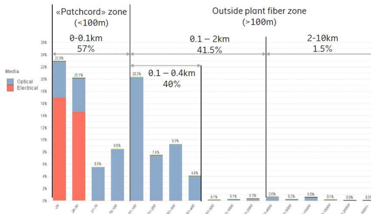
Figure 8: DRAN LLS link length distribution.
