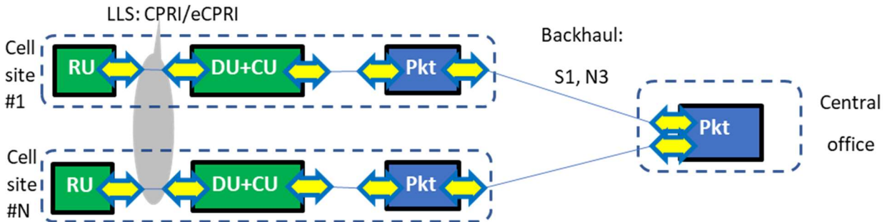
Figure 7: DRAN architecture with RAN nodes, transport nodes and optical pluggables.
