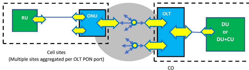
Figure 32: LLS using TDM-PON with separate ONU box.
