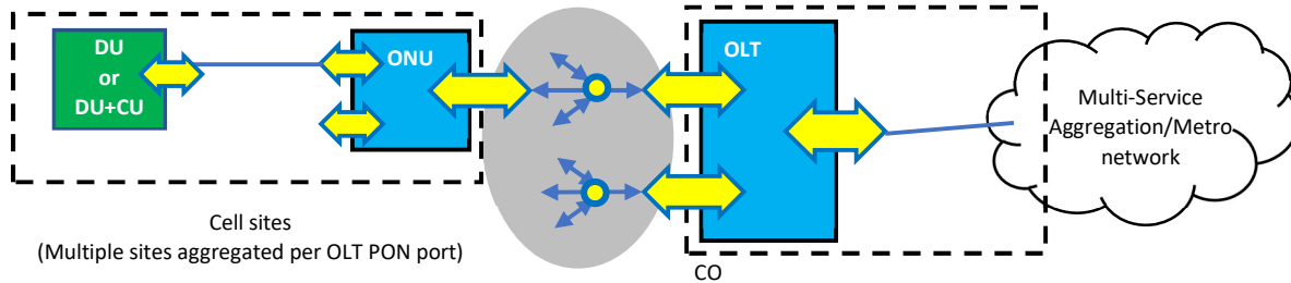
Figure 30 : Up to 20 km Backhaul and HLS with TDM-PON using separate ONU box. HLS is depicted in cases where the CU is centralized. Backhaul is depicted in cases where the CU is located at the cell site.
