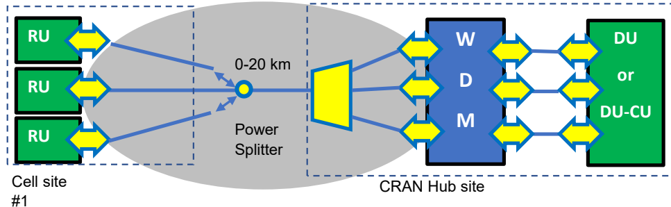
Figure 34: LLS using semi-active DWDM wavelength multiplexed links over a power splitter ODN (WS-WDM-PON).
