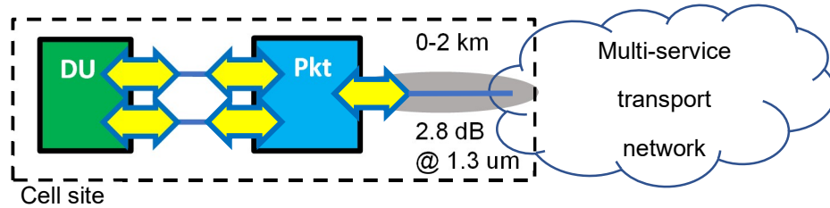
Figure 22: 2 km DRAN intraoffice backhaul direct dual fiber Blueprint. The link specified has a gray background. In cases where the cell site DU is collocated with the CU, backhaul is illustrated. If the CU is located at another location, HLS is illustrated.
