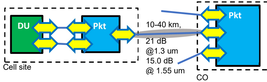
Figure 24: 40 km DRAN backhaul direct parallel fiber, dual or BiDi Blueprint. The link specified has a gray background. In cases where the cell site DU is collocated with the CU, backhaul is illustrated. If the CU is located at another location, HLS is illustrated.
