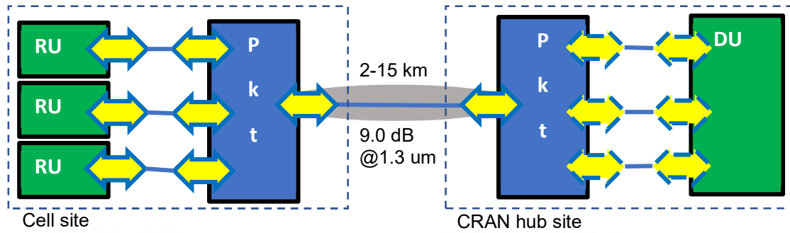
Figure 19: 15 km RU-DU packet multiplexed, P2P or P2MP Blueprint. The link specified has a gray background. There may be additional intermediate Pkt nodes between the depicted Pkt node and DU, for example on case of cloud RAN deployments at the hub site. The intraoffice pluggable at the hub site may be C-temp as indicated by dashed borders.
