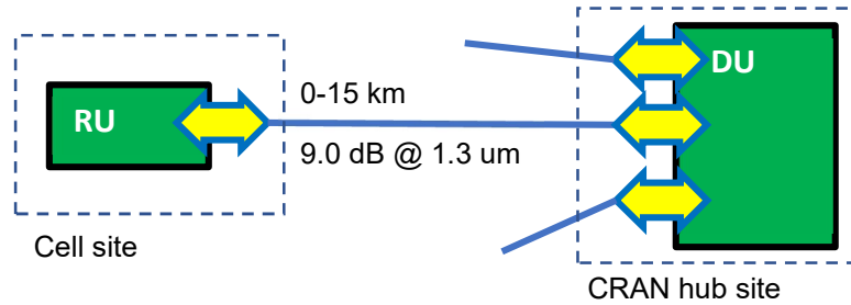
Figure 13: 15 km RU-DU direct parallel fibers Blueprint.
