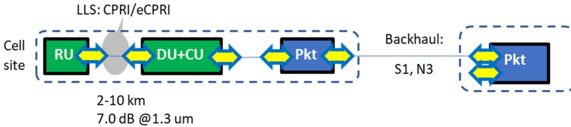
Figure 11: 10 km RU-DU direct parallel fibers Blueprint.
