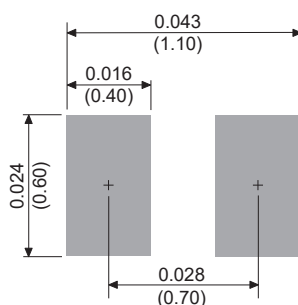
DFN1006-2L
