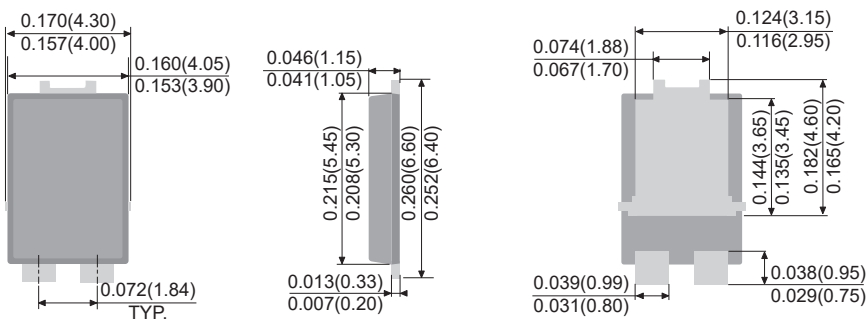
TO-277B
