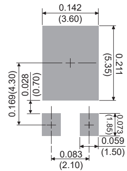
TO-277C
