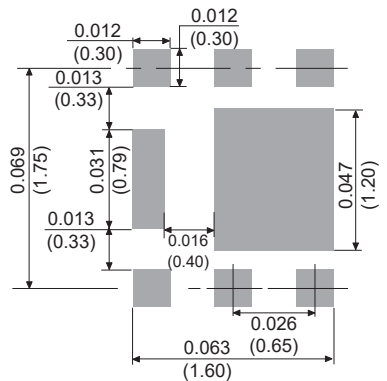
DFN2020-8L
