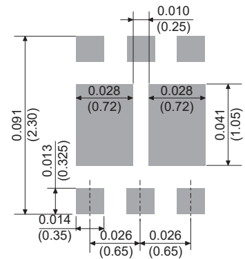
DFN2020B-6L
