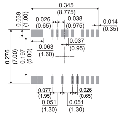
TSSOP-18
