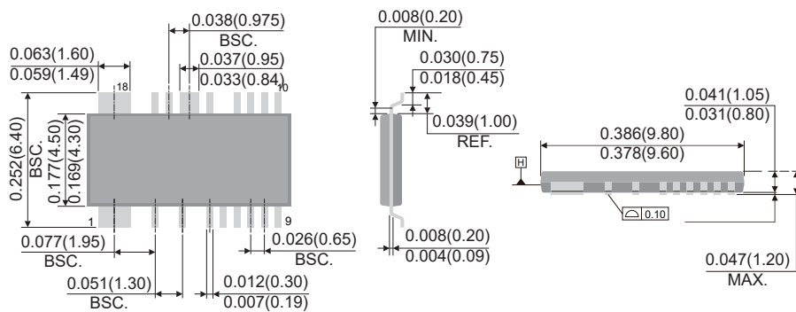
TSSOP-18
