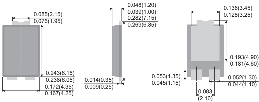
TO-277C
