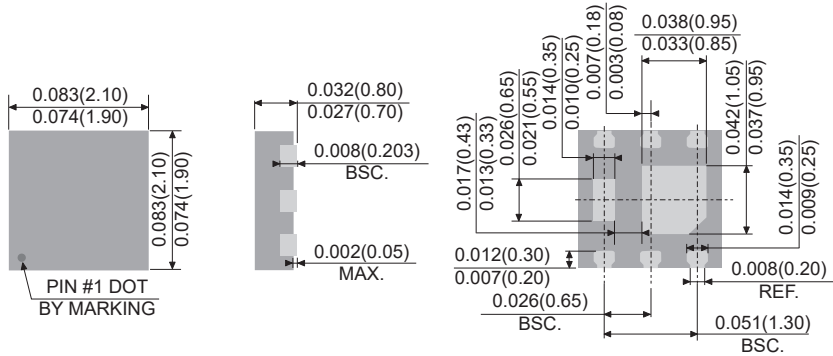
DFN2020-8L
