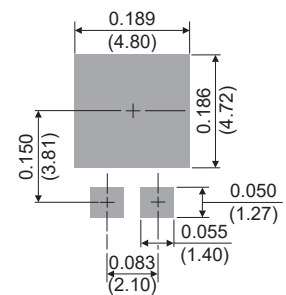
TO-277C
