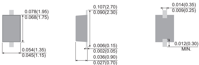
SOD-323S
