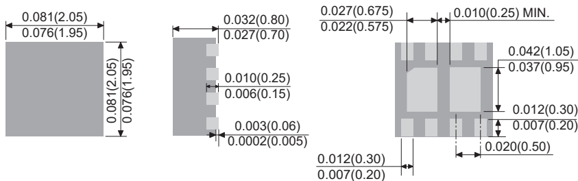
DFN2020-8L
