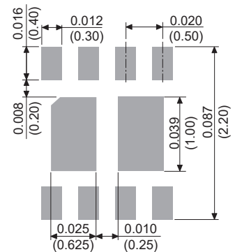
DFN2020-8L
