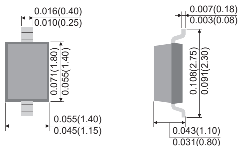
SOD-123HE
