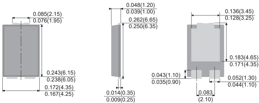
TO-277A
