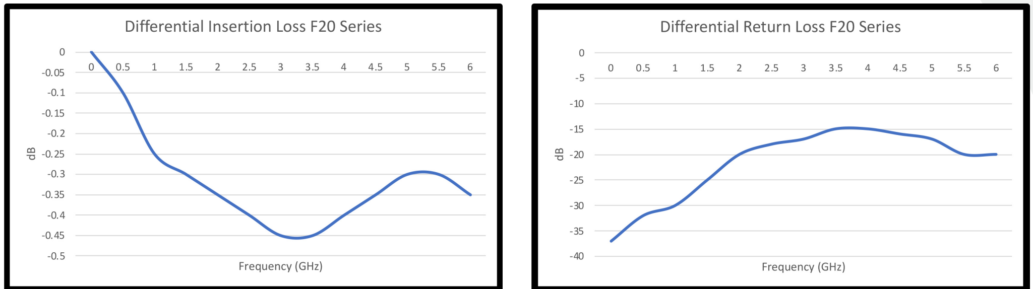
Figure 6: Low-loss performance of FLECTO connectors ensures efficient high-speed transmission (example shows F20 series)
