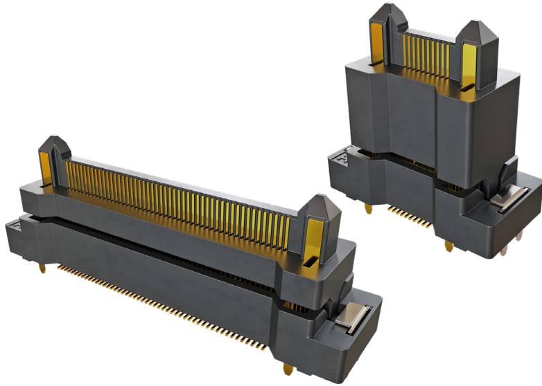
Figure 7: Power contacts also help with blind mating
