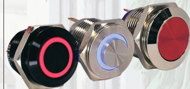
BH Series 16mm or 19mm IP67 Sealing Degree Momentary Panel Mount 2A@36VDC, 1A@125VAC, 0.5A@250VAC
