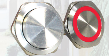
DH22U Series UL Approved 22mm IP67 Sealing Degree Momentary or Latching Panel Mount 3A@ 125VAC, 3A@250VAC
