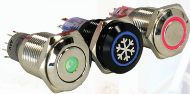
CH Series 16mm IP40 or IP67 Sealing Degree Momentary or Latching Panel Mount 1A@24VDC, 1A@125VAC, 0.5A@250VAC
