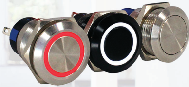
AHU Series 19mm IP67 Sealing Degree Momentary Panel Mount 3A@125VAC, 3A@250VAC
