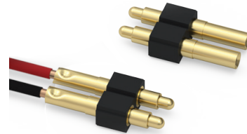
Wire termination
