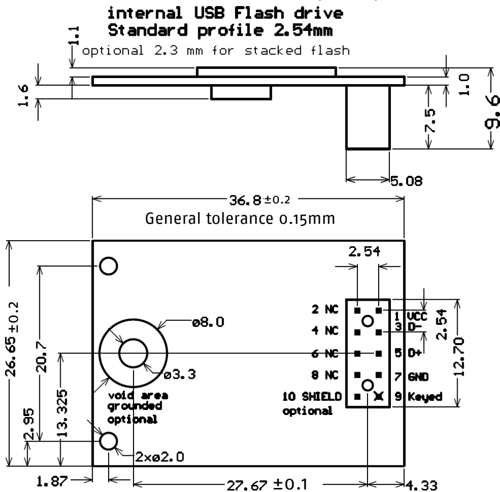
Figure 1: Mechanical Dimensions for 2.54mm connector (standard)
