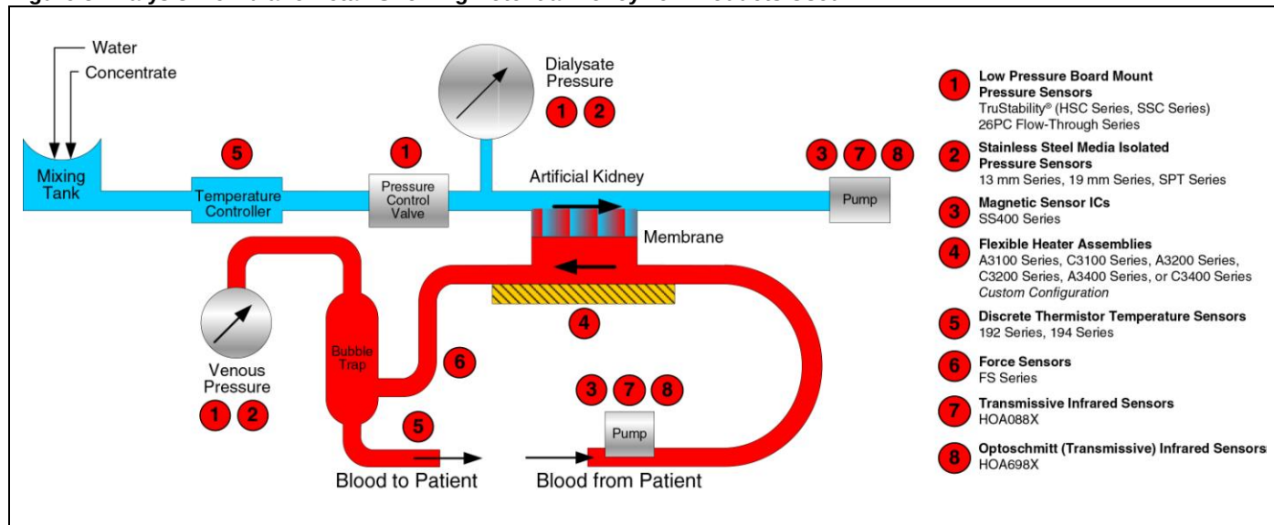
Figure 3. Dialysis Membrane Detail Showing Potential Honeywell Products Used
